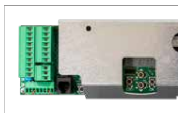
Control unit equipped with connectors and terminals
