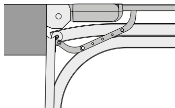
Spring shaft installation
