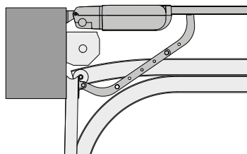
Cross beam installation
